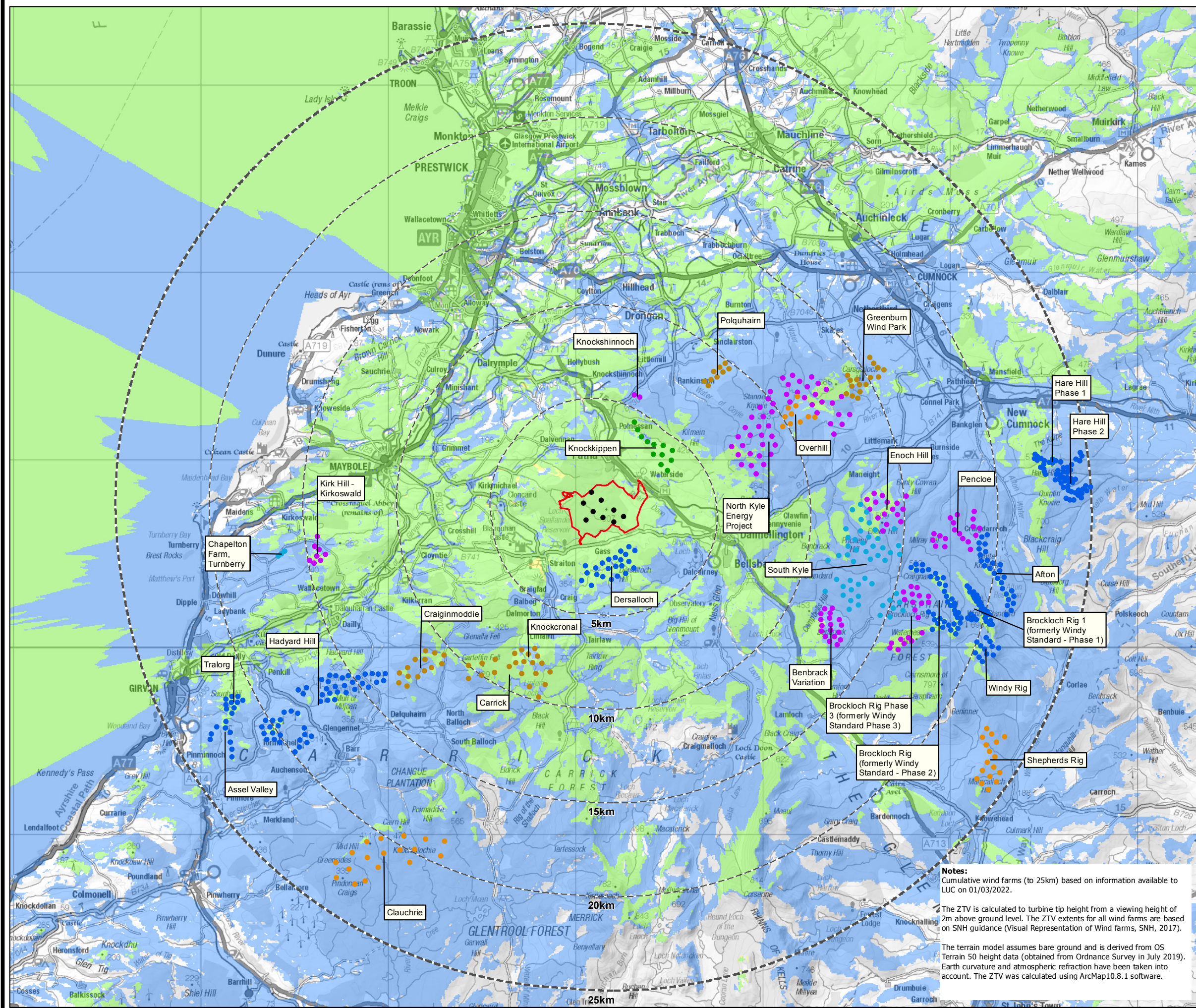
FIGURE 5.1.9c CUMULATIVE ZONE OF THEORETICAL VISIBILITY - OPERATIONAL, CONSENTED AND PROPOSED WIND FARMS AND SCLENTEUCH (25 KM)
