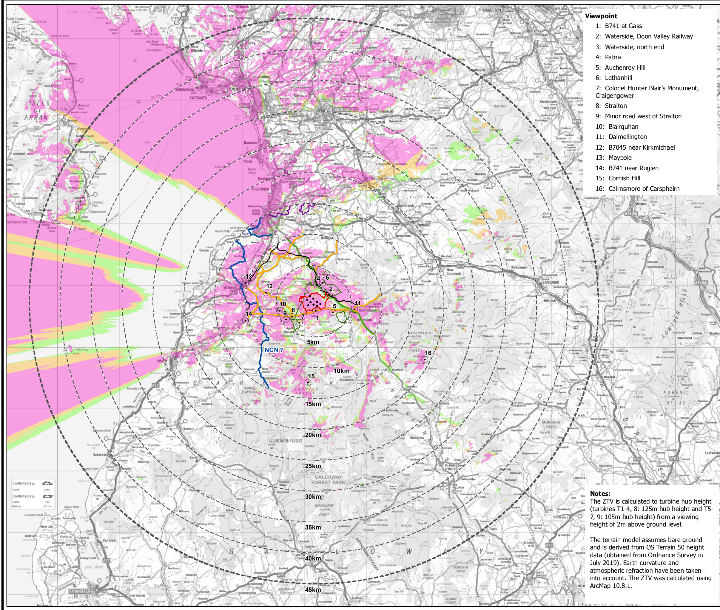
FIGURE 5.1.3a HUB HEIGHT (105M AND 125M) ZONE OF THEORETICAL VISIBILITY (ZTV) AND VIEWPOINT LOCATIONS
